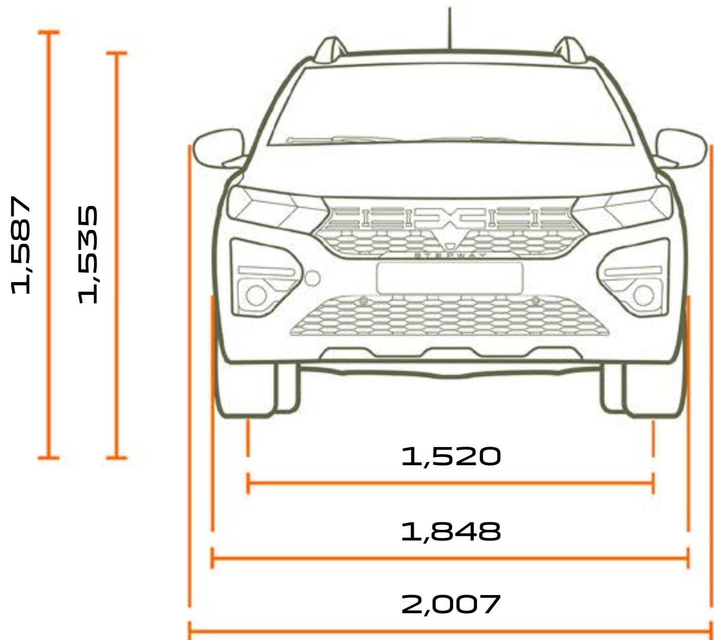
FRONT VIEW
