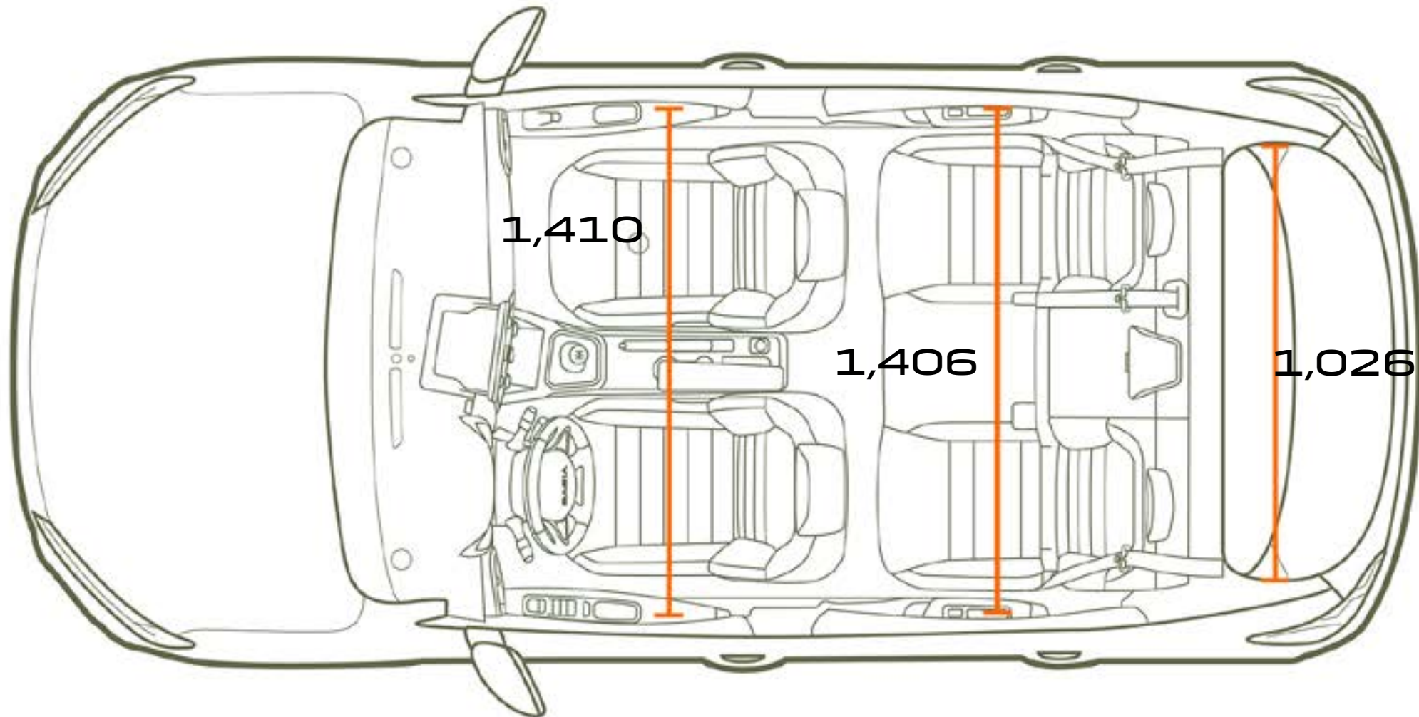
TOP VIEW
